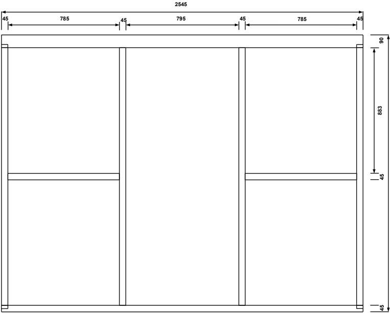
FRONT WALL
