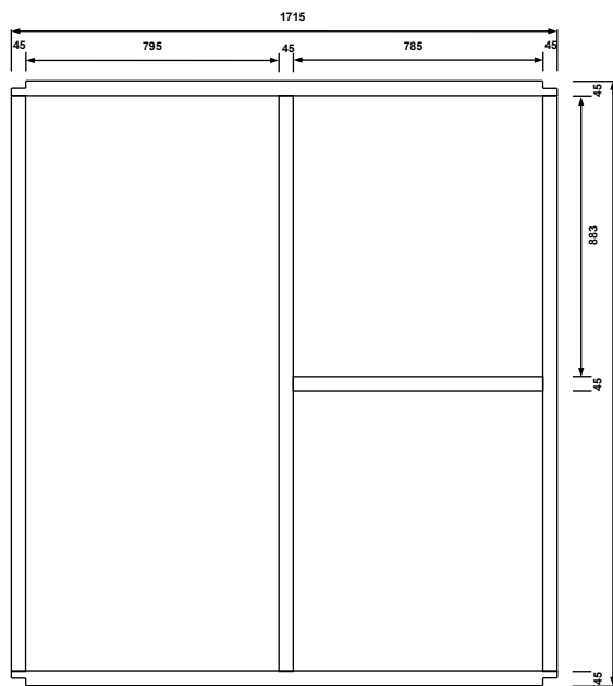
FRONT WALL
