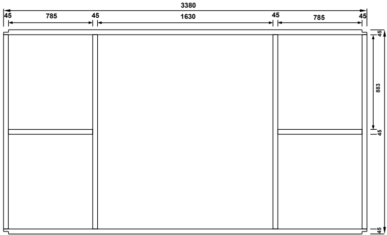
FRONT WALL
