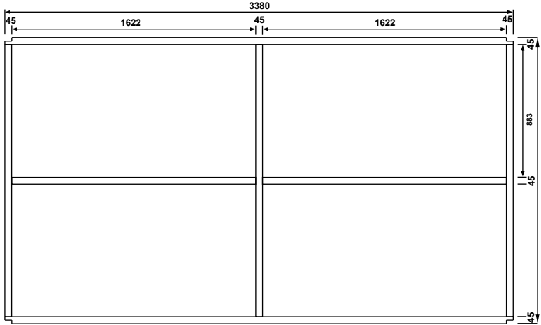
BACK WALL
