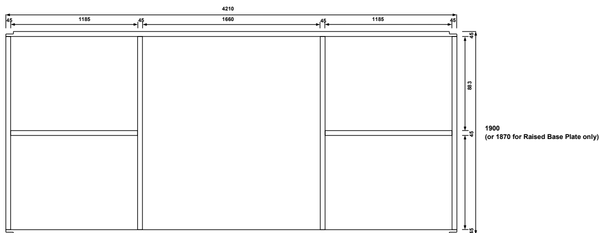
FRONT WALL
