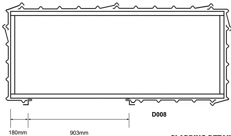
CLADDING DETAIL Birds Eye View
