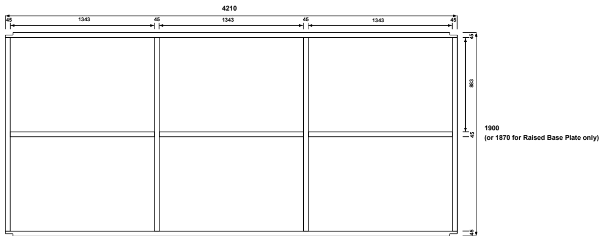
FRONT/BACK WALL
